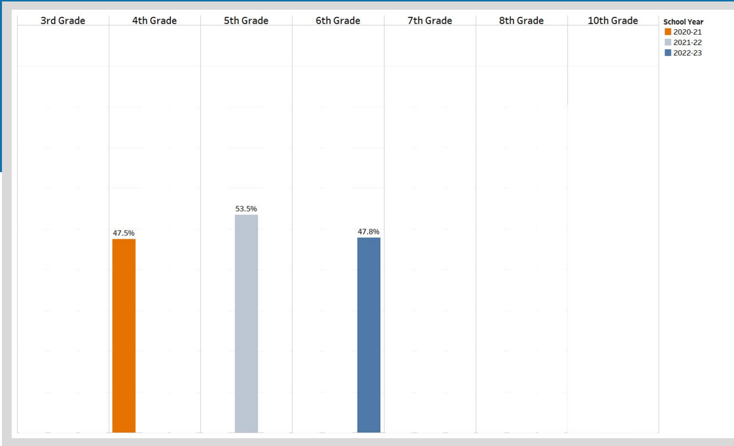
Mathematics Cohort Trend
