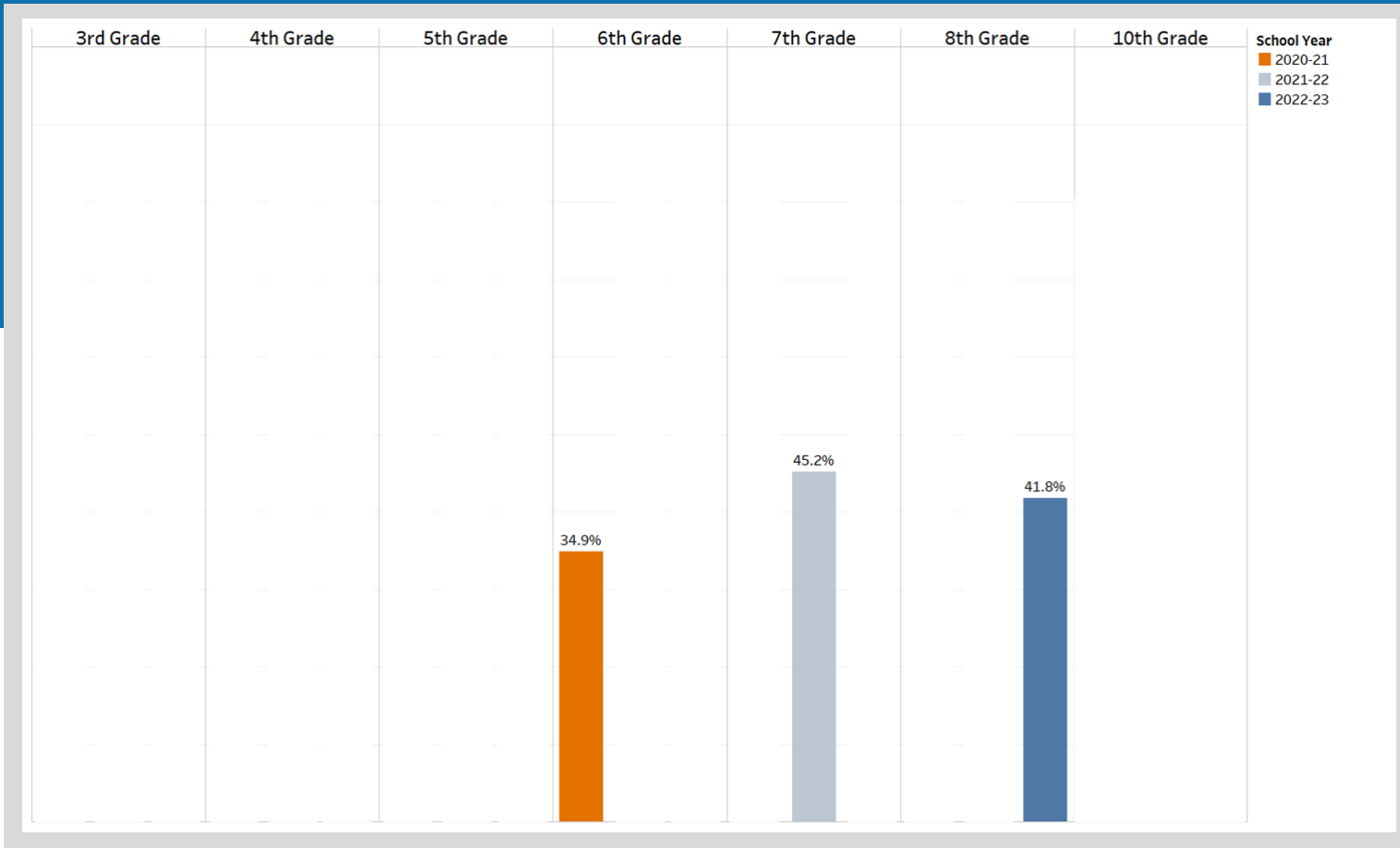
Mathematics Cohort Trend
