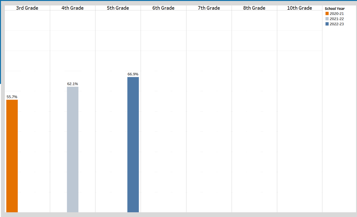
English Language Arts Cohort Trend
